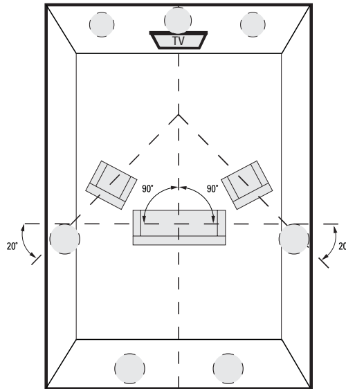
Diagram shows speaker locations for 5.1 and 7.1 systems, when two additional in-ceiling speakers are installed at back of the room.
